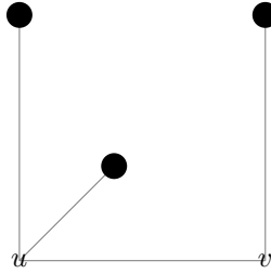
Figure 2: SWEEP rule
