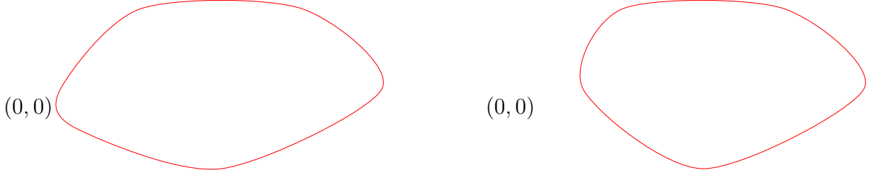
Figure 5: On the left is the Toric Graph. On the right are cross and face checks.
