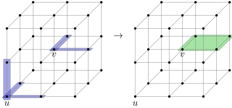
Figure 6: An example of applying the sweep rule, restricted to two vertices, u and v . On the left, the unsatisfied positive checks of u and v are highlighted in blue. On the right, the bits to be flipped are marked in green. Given the syndrome, vertex v flips one of its positive faces, whereas for u , there is no subset of positive faces that, when flipped, decreases the number of local unsatisfied checks. Therefore, u flips no bit.
