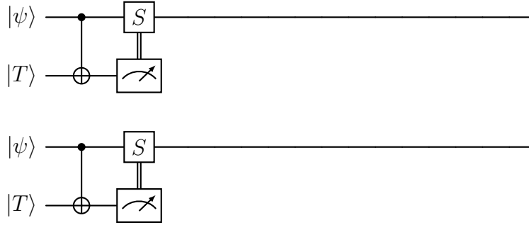
Figure 8: Simulating the T -gate, using the |T\rangle magic state.
