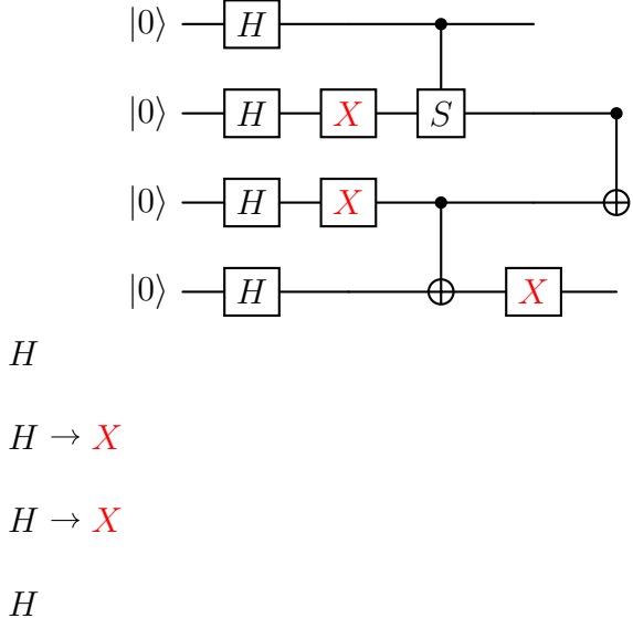
Figure 1: Example of a subjected quantum circuit: the even layers (0, 2, 4) contain the original gates, while the faults are imposed on the odd layers and marked in red.
