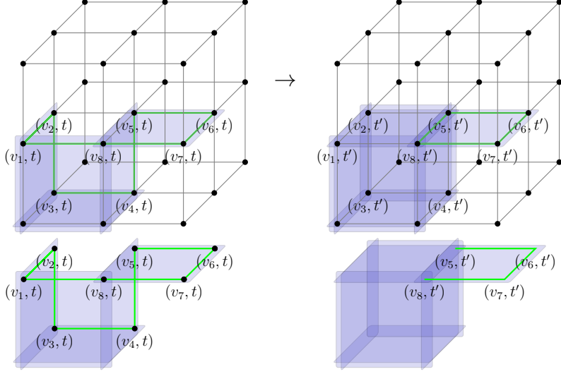
Figure 8: In blue, we have an assignment where the vertex achieving the minimum of L_{d+1} , denoted by v , does not see any unsatisfied checks in its positive local view. The green faces represent an assignment, equivalent to the blue up to stabilizer, such that any local maximum of L_{d+1} (vertices u and w ) sees a non-trivial syndrome in its positive local view.
