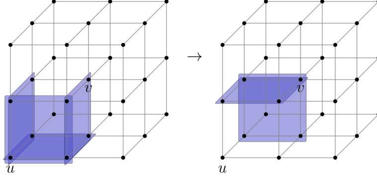
Figure 5: SWEEP rule
