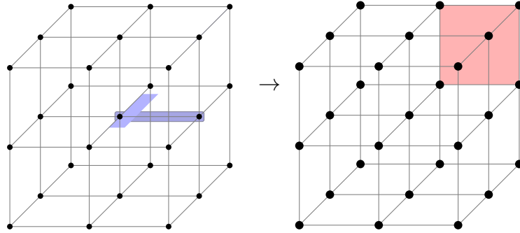
Figure 4: SWEEP rule
