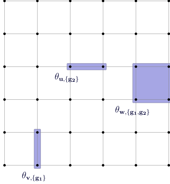
Figure 1: Here we consider a 2D Toric complex. We name the set of generators S = \{g_1, g_2\} , where g_1 is the generator that sends us one step in the north direction, and g_2 sends us in the east direction. For vertices v, u, w , we mark in blue three faces that are rooted at them.
