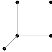
Figure 2: SWEEP rule
