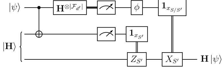
Figure 9: Gate teleportation of the Hadamard gate, using the resource |\mathbf{H}\rangle . We emphasize again that although the Hadamard (at least Hadamard-type) has an O(1) -depth gate realization (at least when d' = d/2 ), we still need all the operations on the quantum register to be strictly transversal for the sake of the proof. Thus, we realize the Hadamard via gate teleportation.
