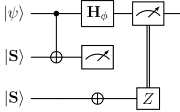
Figure 9: Simulating the \mathbf{S} and \mathbf{T} gates, using the |\mathbf{S}\rangle , |\mathbf{T}\rangle magic states.
