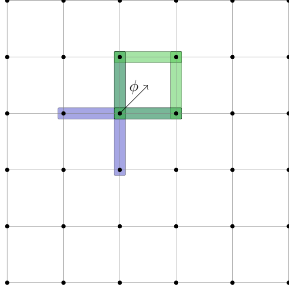
Figure 7: An outline of ???. The \phi -transpose sends Z -stabilizers to X -stabilizers and vice versa. Here we consider the (2, 1) Toric code; namely, the Z -stabilizers (parity checks) are set on the vertices, and the X -stabilizers (phase checks) are set on the squares. In blue and green, we have the edges corresponding to checks \partial^+ \theta_{(2,3),\{\}}^+ and \partial^- \theta_{(2,3),\{(0,1),(1,0)\}}^- . The example shows that indeed \phi maps between the two.
