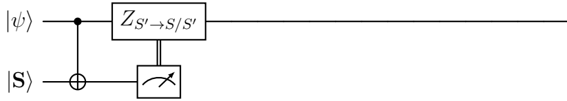
Figure 1: Simulating the S -gate, using the |\mathbf{S}\rangle magic state.
