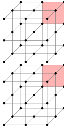
Figure 1: SWEEP rule
