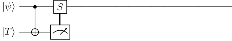
Figure 8: Simulating the T -gate, using the |T\rangle magic state.
