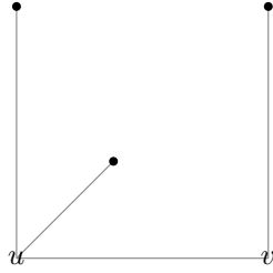
Figure 2: SWEEP rule
