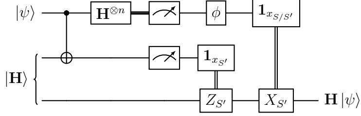
Figure 9: Gate teleportation of the Hadamard gate, using the resource |\mathbf{H}\rangle . We emphasize again that although the Hadamard 8 has an O(1) -depth gate realization, we still need all the operations on the quantum register to be strictly transversal for the sake of the proof. Thus, we realize the Hadamard via gate teleportation.
