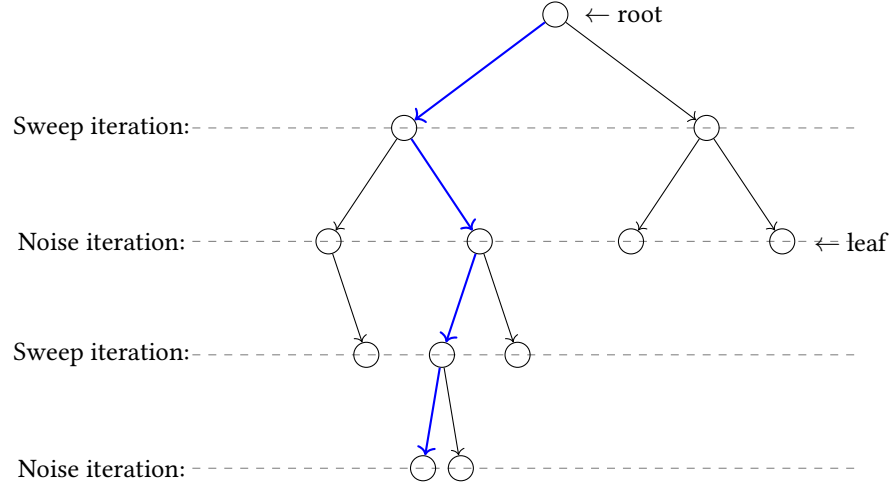
Figure 3: blabla
