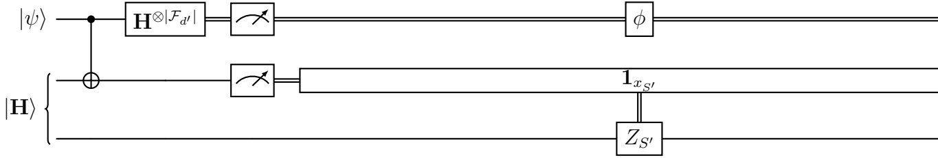
Figure 10: Gate teleportation of the Hadamard gate, using the resource |\mathbf{H}\rangle . We emphasize that although the Hadamard (at least Hadamard-type) has an O(1) -depth gate realization (at least when d' = d/2 ), we still need all the operations on the quantum register to be strictly transversal for the sake of the proof. Thus, we realize the Hadamard via gate teleportation.
