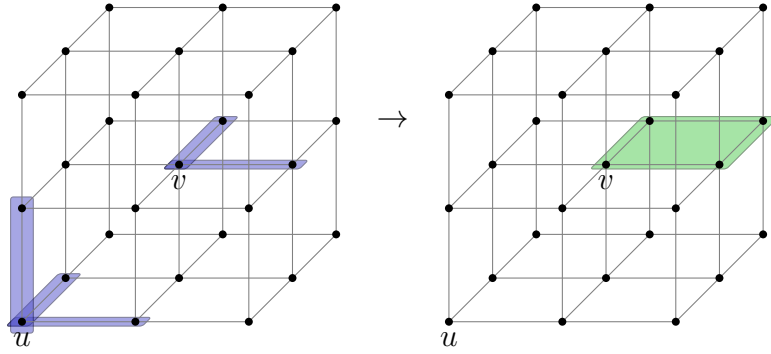
Figure 4: SWEEP rule
