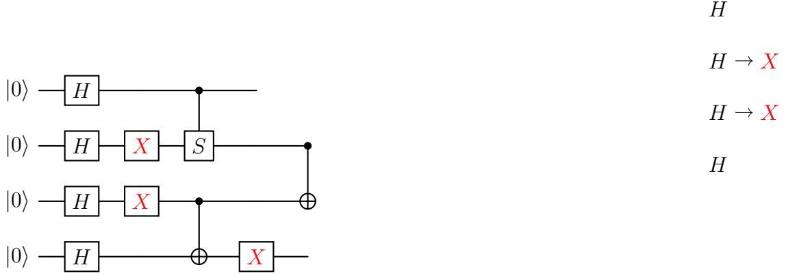
Figure 1: Example of a subjected quantum circuit: the even layers (0, 2, 4) contain the original gates, while the faults are imposed on the odd layers and marked in red.
