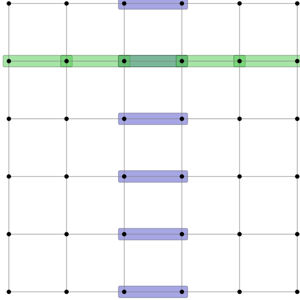
Figure 7: In blue and green are the binary presentations x_S and z_S of logical code words of the (2, 1) -Toric code. The edge \{(5, 4), (0, 4)\} is omitted for clarity (it should be a green edge that hovers over the green line).
