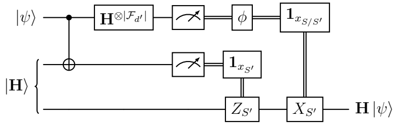
Figure 10: Gate teleportation of the Hadamard gate, using the resource |\mathbf{H}\rangle . We emphasize that although the Hadamard (at least Hadamard-type) has an O(1) -depth gate realization (at least when d' = d/2 ), we still need all the operations on the quantum register to be strictly transversal for the sake of the proof. Thus, we realize the Hadamard via gate teleportation.
