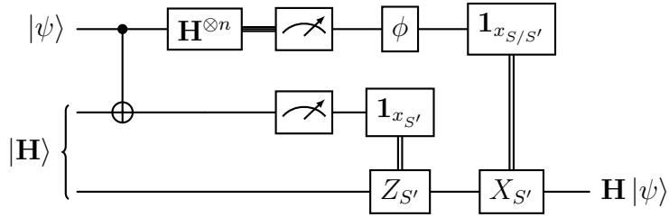
Figure 9: Gate teleportation of the Hadamard gate, using the resource |\mathbf{H}\rangle . We emphasize again that although the Hadamard (at least Hadamard-type) has an O(1) -depth gate realization, we still need all the operations on the quantum register to be strictly transversal for the sake of the proof. Thus, we realize the Hadamard via gate teleportation.
