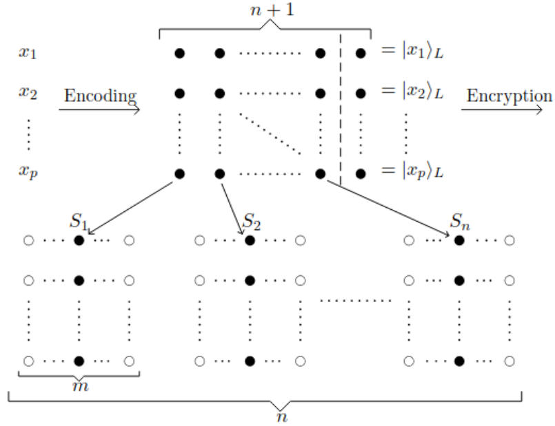
Figure 5: Skechth of the encryption scheme, taken form [NS17]
