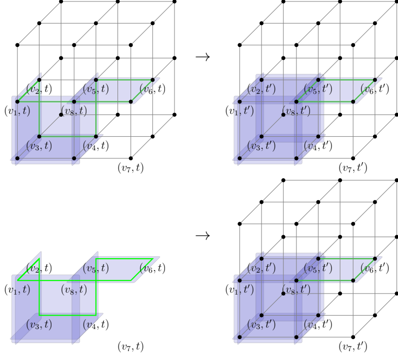
Figure 8: In blue, we have an assignment where the vertex achieving the minimum of L_{d+1} , denoted by v , does not see any unsatisfied checks in its positive local view. The green faces represent an assignment, equivalent to the blue up to stabilizer, such that any local maximum of L_{d+1} (vertices u and w ) sees a non-trivial syndrome in its positive local view.
