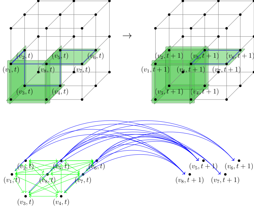
Figure 8: Above: The application of a sweep-cycle, where the green faces represent the bits assignment z , and the blue edges correspond to unsatisfied checks \partial z . The vertices in \partial z are labeled as v_1, v_2, \dots, v_8 . Below: The Toom's contour derived from the single computation layer that matches the cycle. Arrows are colored in blue, while forks are colored in green. Note that (v_1, t+1) doesn't belong to the Toom's contour (since v_1 doesn't belong to the syndrome at time t+1 ).
