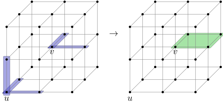
Figure 6: An example of applying the sweep rule within the (3,2) -Toric code. In the (3,2) -Toric code, bits are placed on the squares and Z -stabilizers (parity checks) on the edges. The view is restricted to two vertices, u and v . On the left, the unsatisfied positive checks of u and v are highlighted in blue. On the right, the bits to be flipped are marked in green. Given the syndrome, vertex v flips one of its positive faces, whereas for u , there is no subset of positive faces that, when flipped, decreases the number of local unsatisfied checks. Therefore, u flips no bit.
