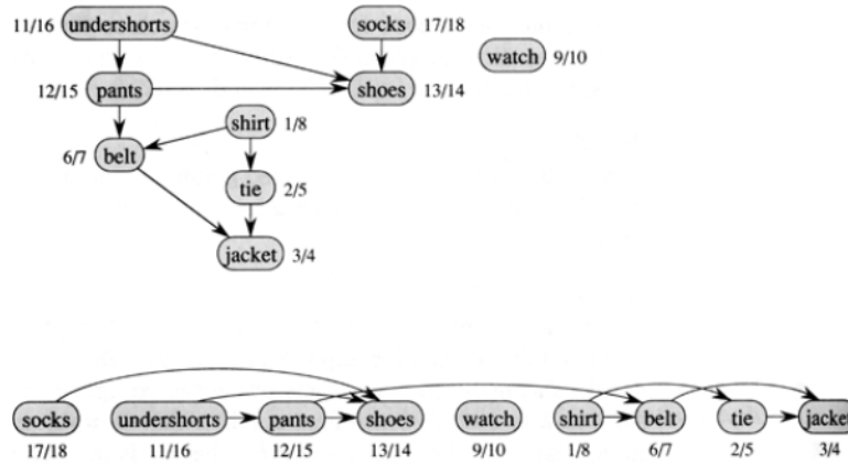
Figure 5.1: Topological sort
