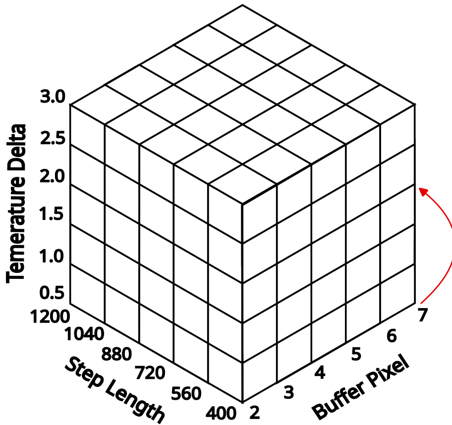
Abb. 3-7: Visual depiction of the second Morris sampling grid, spanning step length, buffer pixel count, and the temperature delta threshold. The red arrow indicates the delta chosen.
