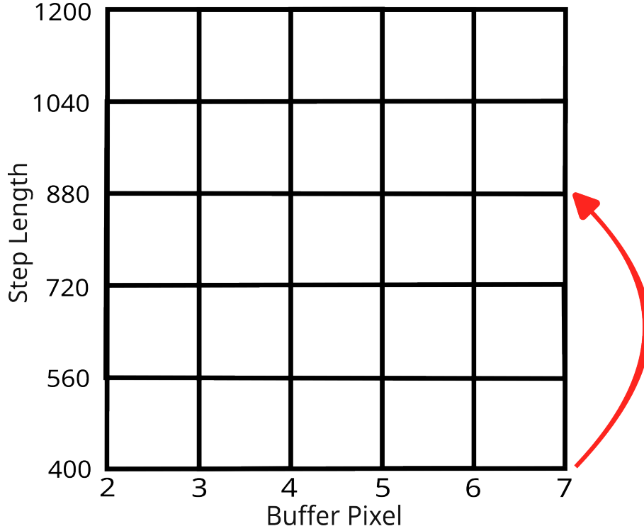
Abb. 3-2: Visual depiction of the Morris sampling grid, spanning step length and buffer pixel count. The arrow shows the \Delta picked for the morris experiment, which is a jump of 3 cells.
