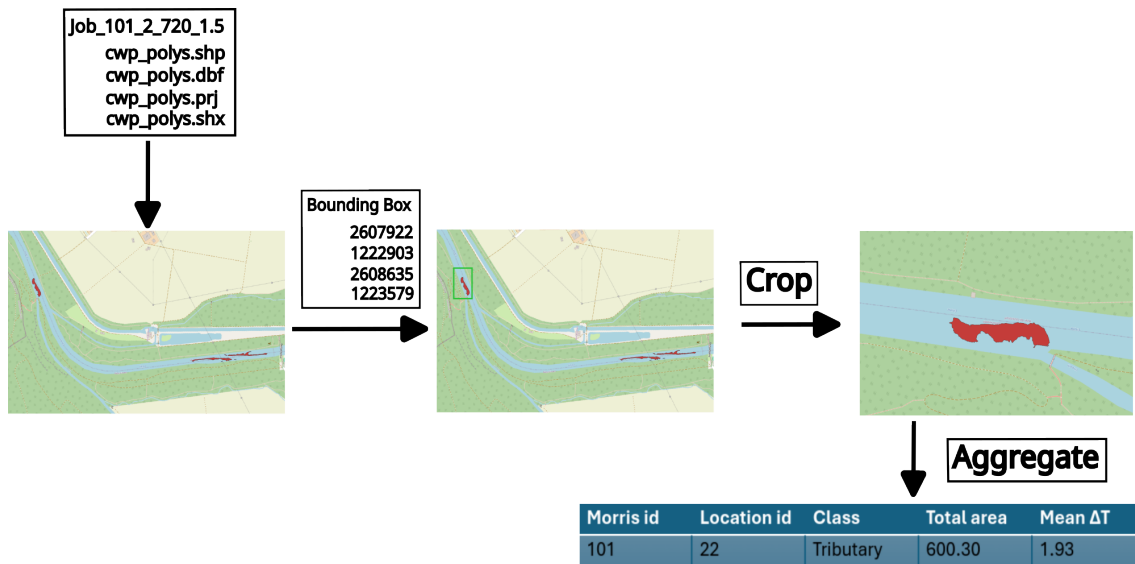
Abb. 3-8: Schematic overview of the lumped-statistics computation for one annotated CWP location (Limpbach inflow into the Emme near Utzenstorf BE). For each Morris run, CWP polygons are cropped to the bounding box; if polygons are present, total area and area-weighted mean temperature delta are computed; if the bounding box is empty, both are set to zero.
