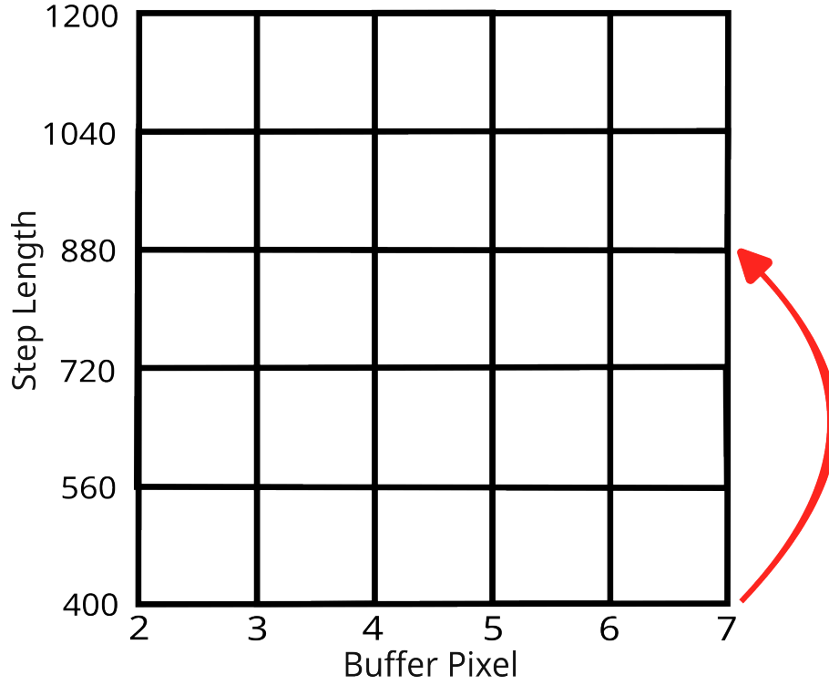
Abb. 3-3: Visual depiction of the Morris sampling grid, spanning step length and buffer pixel count.
