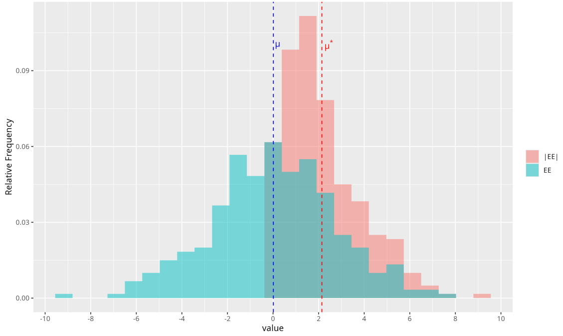
Abb. 2-4: The difference of \mu and c visualized with their underlying distribution \mathcal{G} and \mathcal{F} . While the mean \mu of the distribution \mathcal{F} lies at around zero, \mu^* significantly deviates from zero
