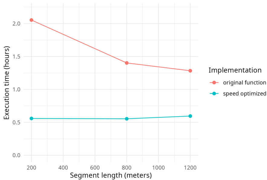
Abb. 1-1: Execution time of the original (v1) and optimized (v2) implementations of detect_cwp_single as a function of segment length. The optimized implementation shows execution times that are both shorter and largely constant across segment lengths, whereas the original implementation scales disproportionately with decreasing segment length (i.e., increasing number of segments).
