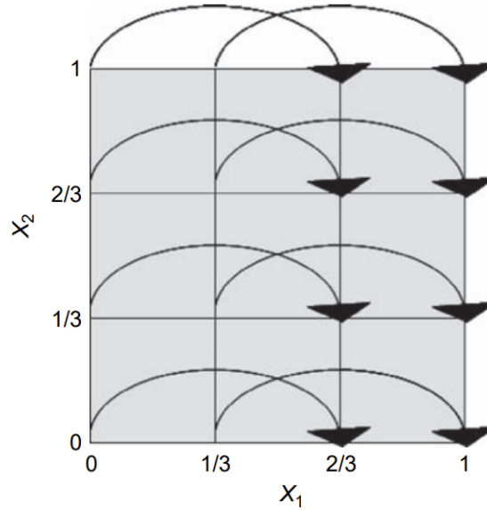
Abb. 2-1: An example grid \Omega . The grid features two parameters X_1, X_2 , meaning that it is a two-dimensional grid. Further, it features four levels ( p = 4 ). The step length \Delta chosen here is \frac{2}{3} , which corresponds to an element of the set of viable values for \Delta : 1 - \frac{1}{4-1} = 1 - \frac{1}{3} = \frac{2}{3} .
