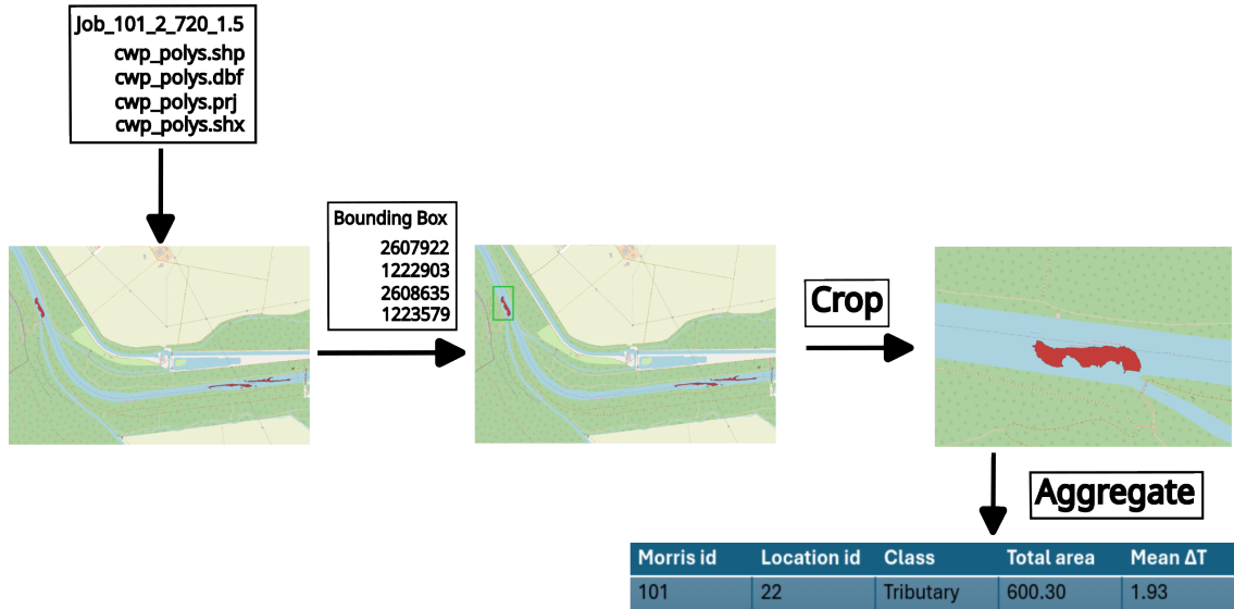
Abb. 4-7: Schematic overview of the lumped-statistics computation for one annotated CWP location (Limpbach inflow into the Emme near Utzenstorf BE). For each Morris run, CWP polygons are cropped to the bounding box; if polygons are present, total area and area-weighted mean temperature delta are computed; if the bounding box is empty, both are set to zero.
