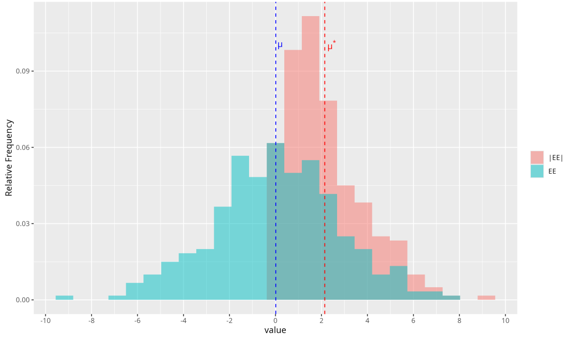
Abb. 2-4: The difference of \mu and \mu^* visualized with their underlying distribution \mathcal{F}_i and \mathcal{G}_i . While the mean \mu of the distribution \mathcal{F}_i lies at around zero, \mu^* significantly deviates from zero.
