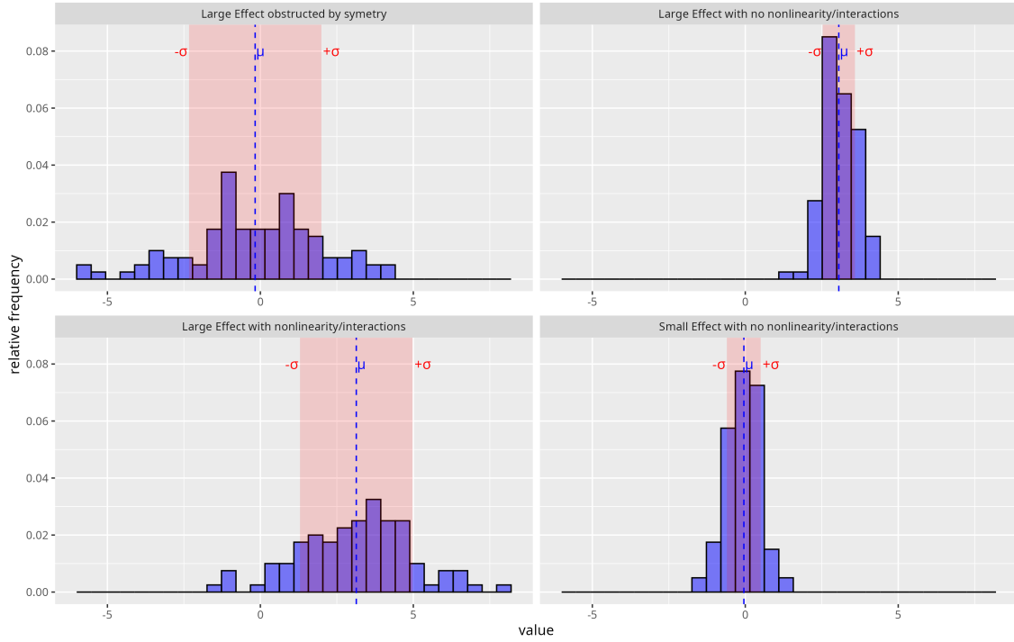
Abb. 2-3: Four example distributions \mathcal{F}_i of a parameter X_i , illustrating how \mu and \sigma jointly characterise parameter influence. Top left: a large effect obscured by symmetry. Top right: a large effect with no nonlinearity or interactions. Bottom left: a large effect with nonlinearity or interactions. Bottom right: a small effect with no nonlinearity or interactions.
