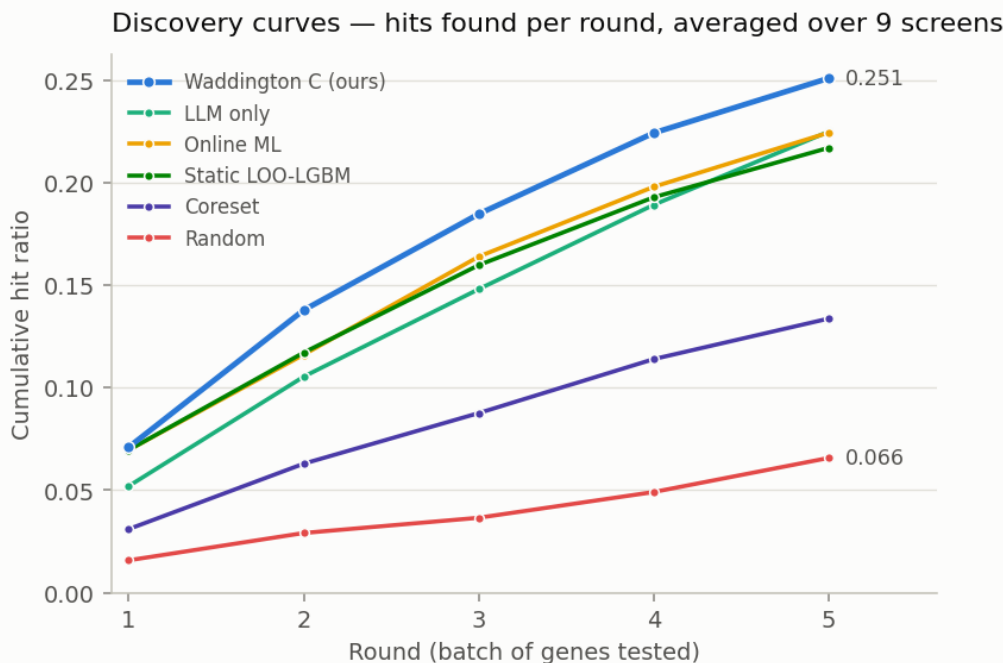
Figure 1: Discovery curves: cumulative hit ratio per round, averaged over the nine screens, for the final leakage-free Waddington (5 seeds, hit@R5 0.251). The hybrid separates from every baseline from round 2 onwards. Per-screen values are given in Figure 3; no error band is drawn because the spread across screens is dominated by how hard each screen is (K562-Essential 0.56 vs. Carnevale22 0.06), which would encode screen difficulty rather than uncertainty about a method.
