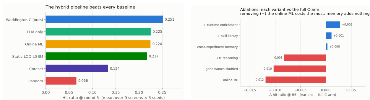
Figure 2: Left: average hit ratio @ R5 per method, final leakage-free Waddington 0.251 (Table 4). Right: paired ablation deltas (Table 7) — a legacy configuration analysis (variants share the legacy routed C-arm reference, statistically identical to the final system). Colour states a fact about the variant (it scored lower than the full arm), not a verdict on the component: a red “– online ML” means removing online ML costs 0.012, i.e. it is the most valuable part.
