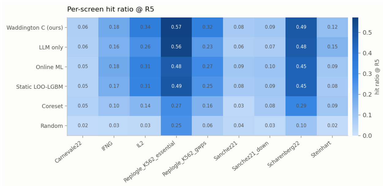
Figure 3: Per-screen hit ratio at round 5 for every method.
