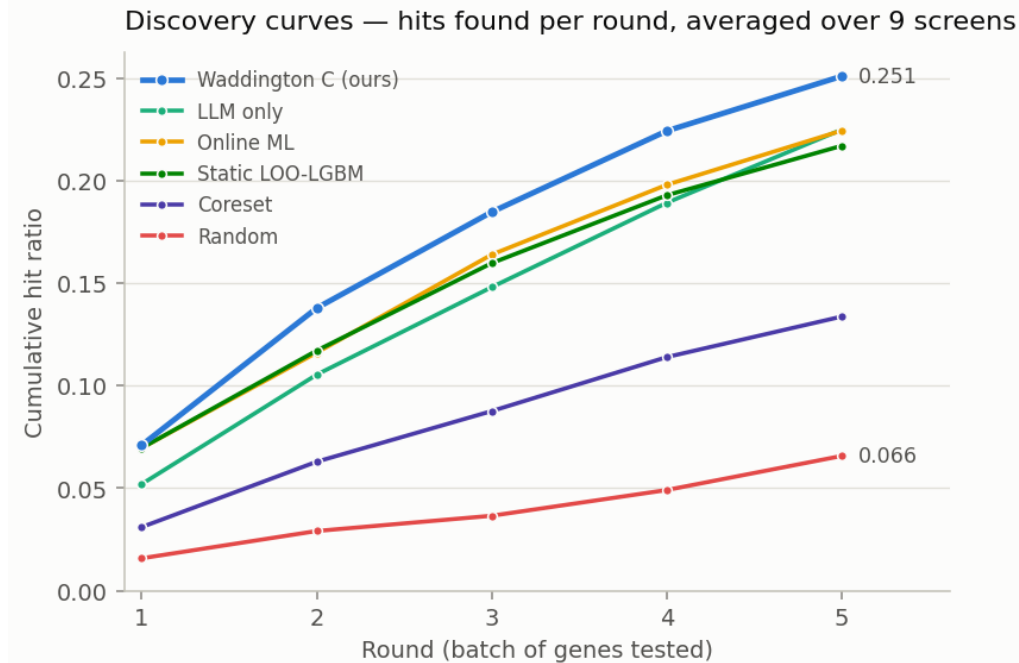
Figure 1: Discovery curves: cumulative hit ratio per round, averaged over the nine screens, for the final leakage-free Waddington (5 seeds, hit@R5 0.251). The hybrid separates from every baseline from round 2 onwards. Per-screen values are given in Figure 3; no error band is drawn because the spread across screens is dominated by how hard each screen is (K562-Essential 0.56 vs. Carnevale22 0.06), which would encode screen difficulty rather than uncertainty about a method.
