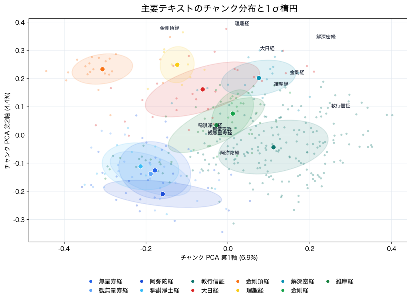
Figure3: Chunk distributions and one-standard-deviation ellipses for major texts. Small points are chunks and darker points are chunk centroids for each text. Because the explained variance of the two-dimensional PCA is low, overlap should be interpreted together with high-dimensional neighbor-mixing measures.
