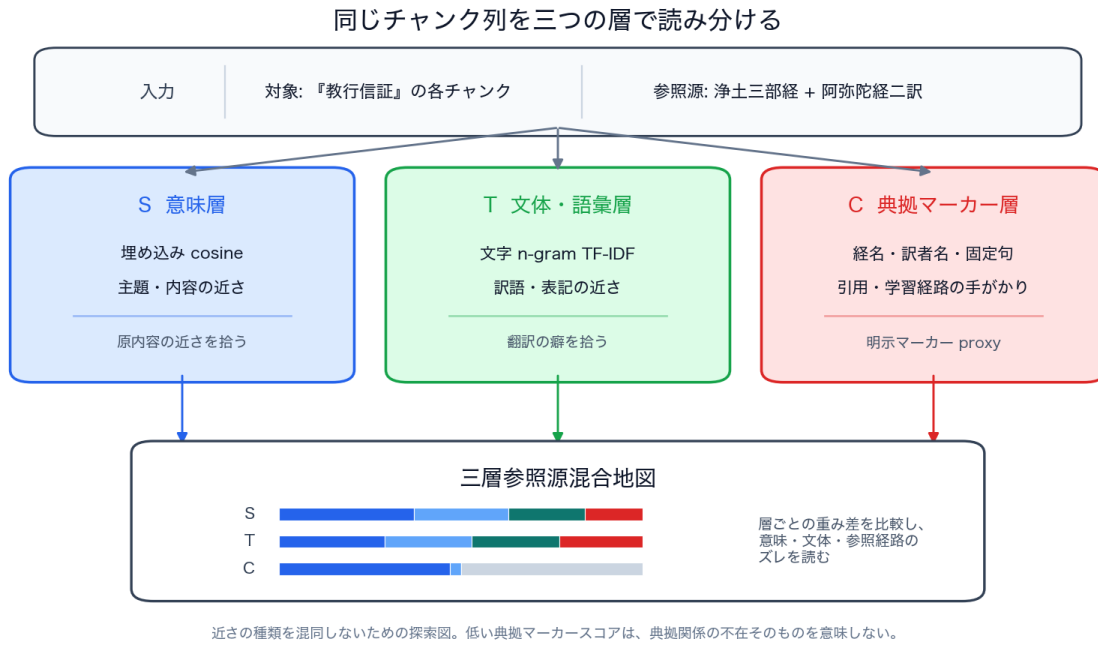
Figure1: Conceptual diagram of the three-layer source-mixture map. The same target chunk sequence is read through the semantic, stylistic/lexical, and source-marker layers, and the differences among layer-specific weights are interpreted as differences in kinds of proximity. The source-marker layer is not a complete detector of quotation or reference; it is an exploratory proxy based on explicit markers.
