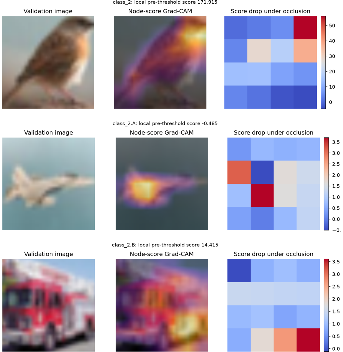
Figure 6. Width-16, seed-17 bird-vs-rest tree: parent, positive child A , and negative child B . The parent map emphasizes the bird’s upper body/head. The B example is a truck, which is compatible with learning to suppress a bird false positive, but a high local score alone does not establish that this particular validation image was actually corrected by the full tree.
