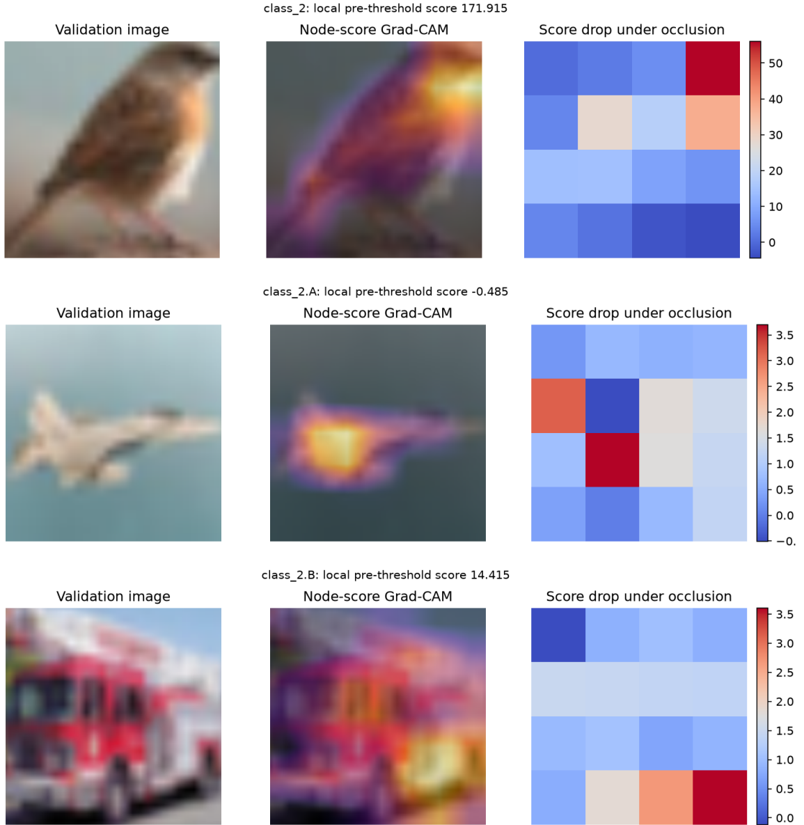
Figure 4. Width-16, seed-17 bird-vs-rest tree: parent, positive child A , and negative child B . The parent map emphasizes the bird’s upper body/head. The B example is a truck, which is compatible with learning to suppress a bird false positive, but a high local score alone does not establish that this particular validation image was actually corrected by the full tree.
