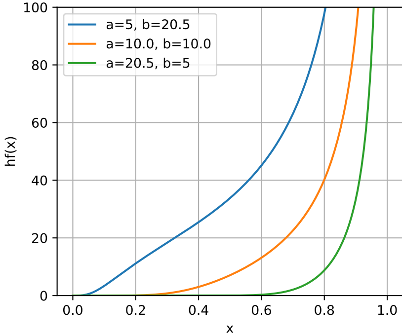
Beta distribution: hazard function
