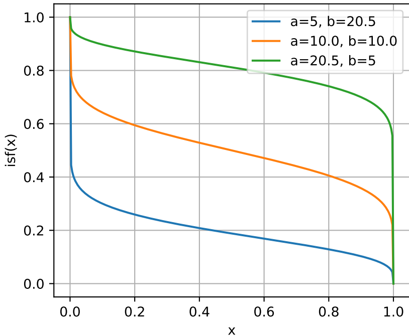
Beta distribution: inverse survival function
