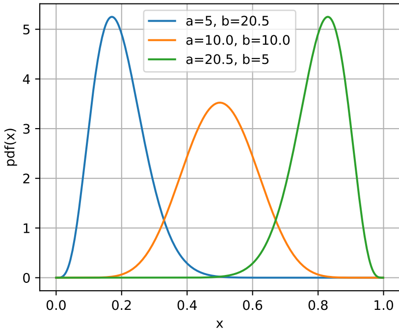
Beta distribution: pdf
