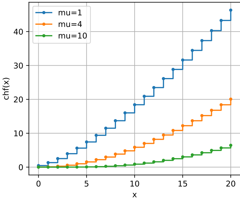
Poisson distribution: cumulative hazard function
