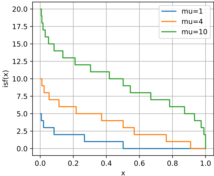
Poisson distribution: inverse survival function
