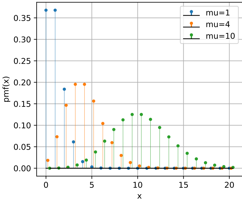
Poisson distribution: pmf
