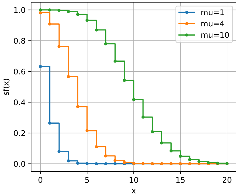
Poisson distribution: survival function
