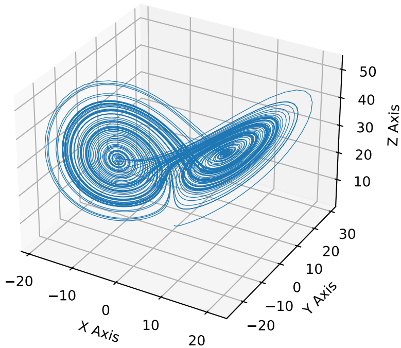
Lorenz Attractor
