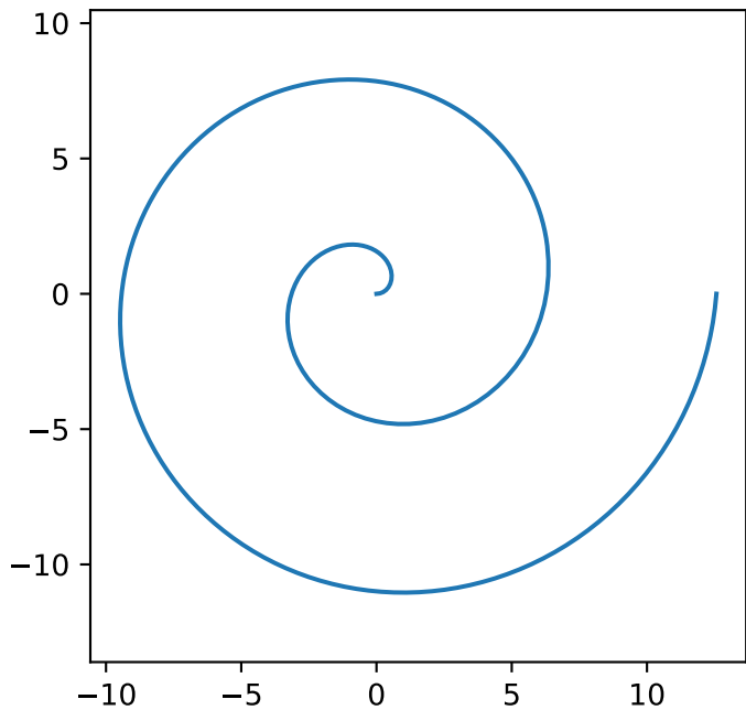
Archimedes Spiral
