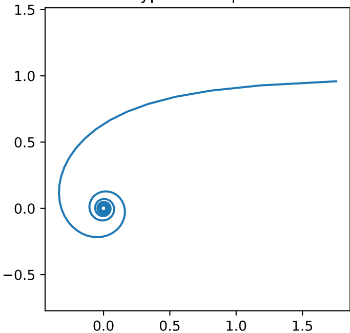
Hyperbolic Spiral
