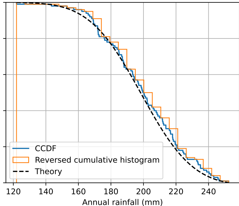
Cumulative distributions
