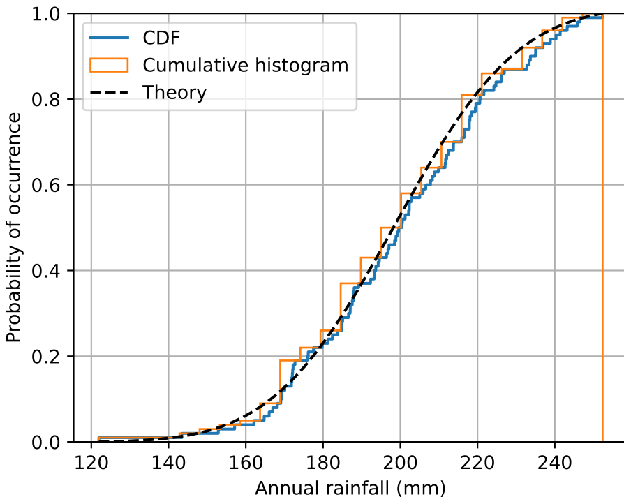
Cumulative distributions
