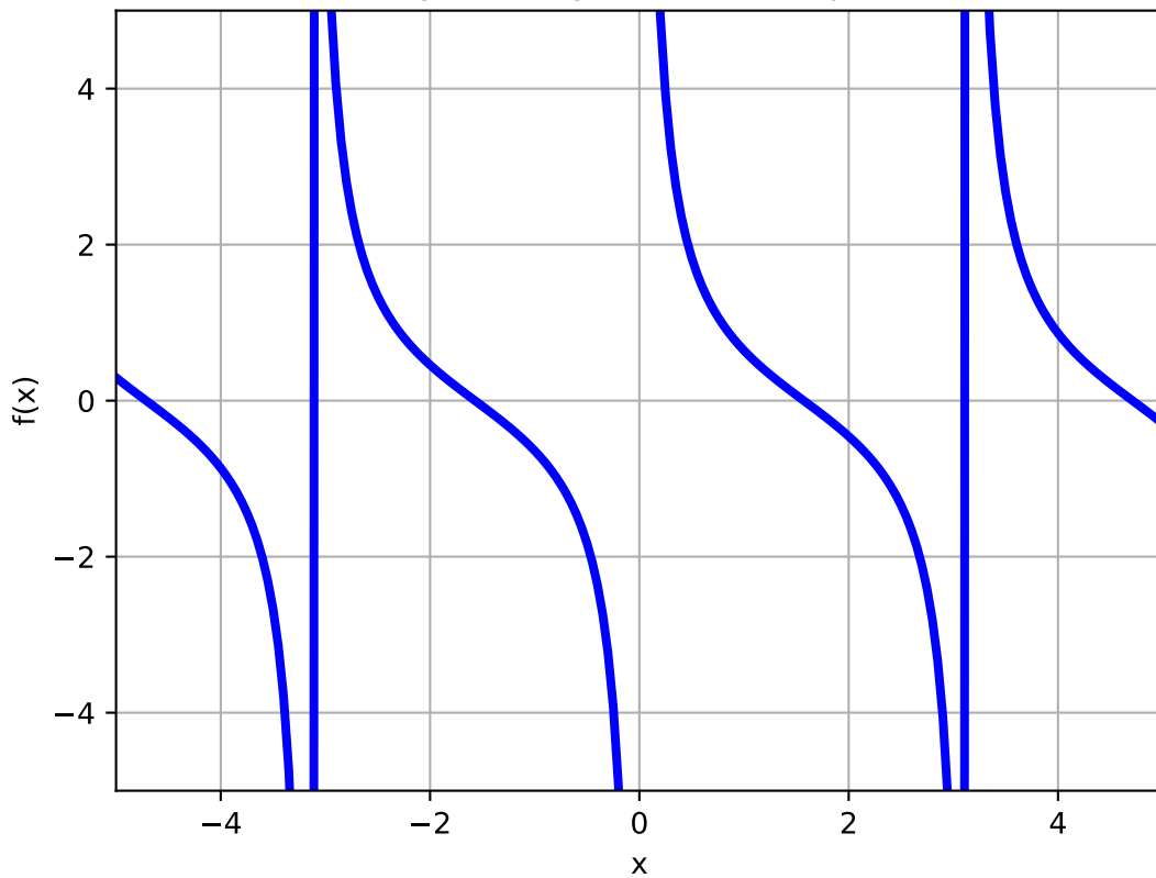
Cotangent, singularities not specified
