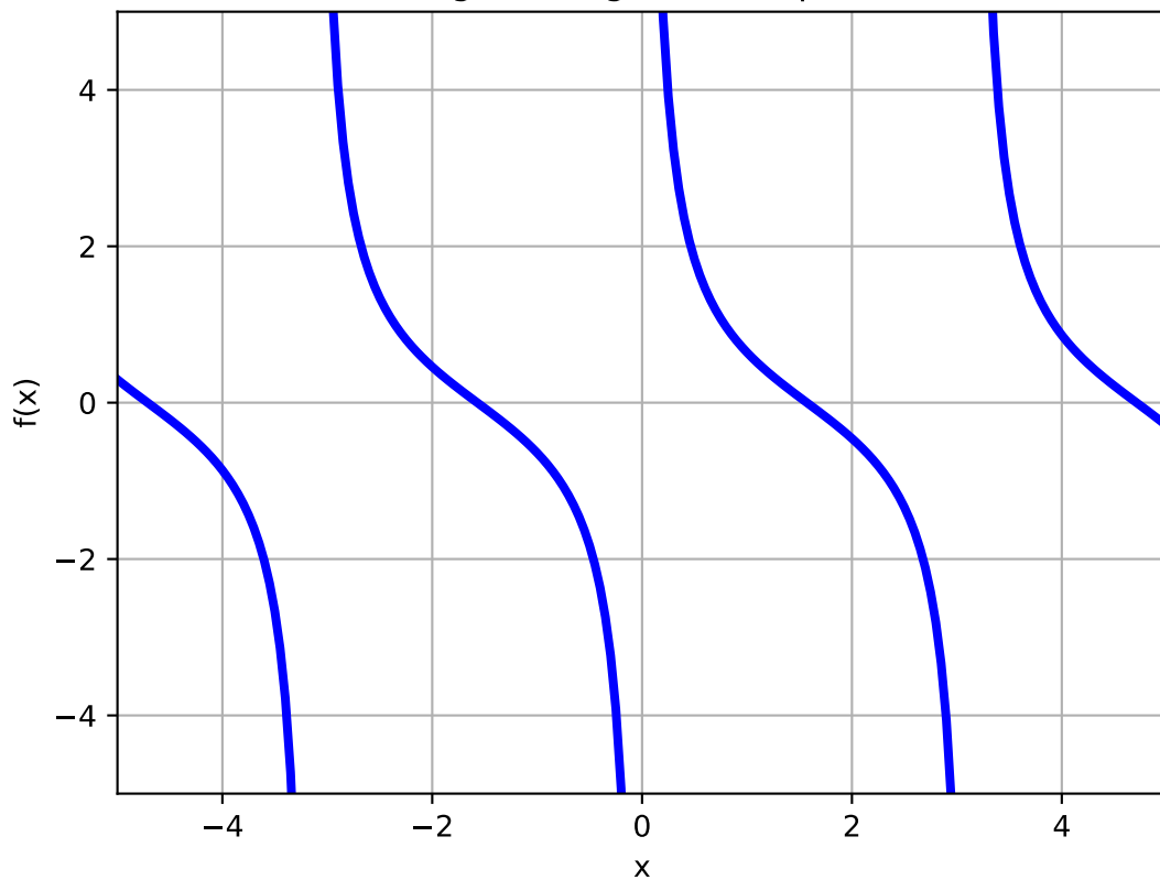
Cotangent, singularities specified
