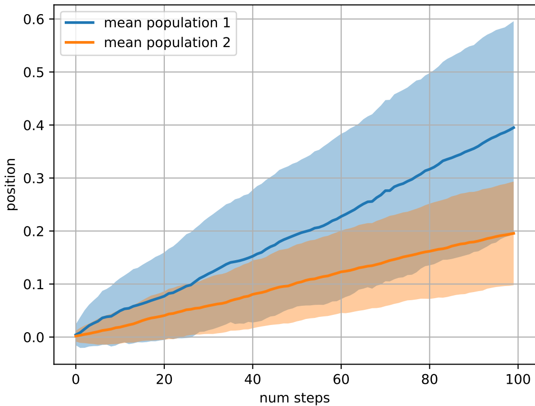
random walkers empirical \mu and \pm\sigma interval
